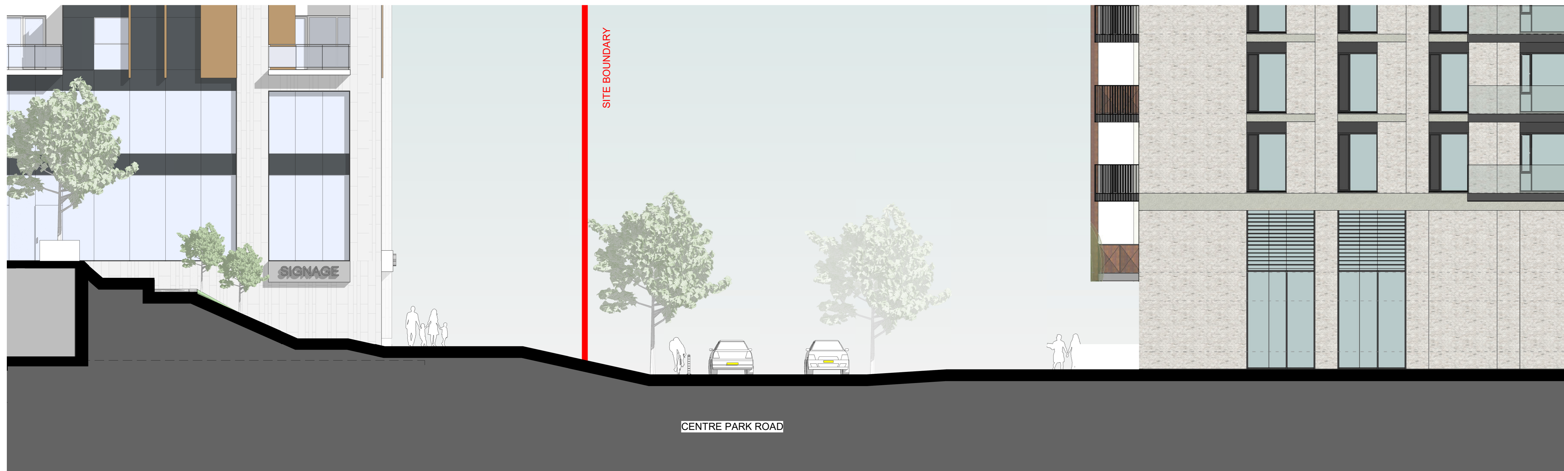
3 CONTEXTUAL SITE SECTION L-L - DETAIL 1:100
