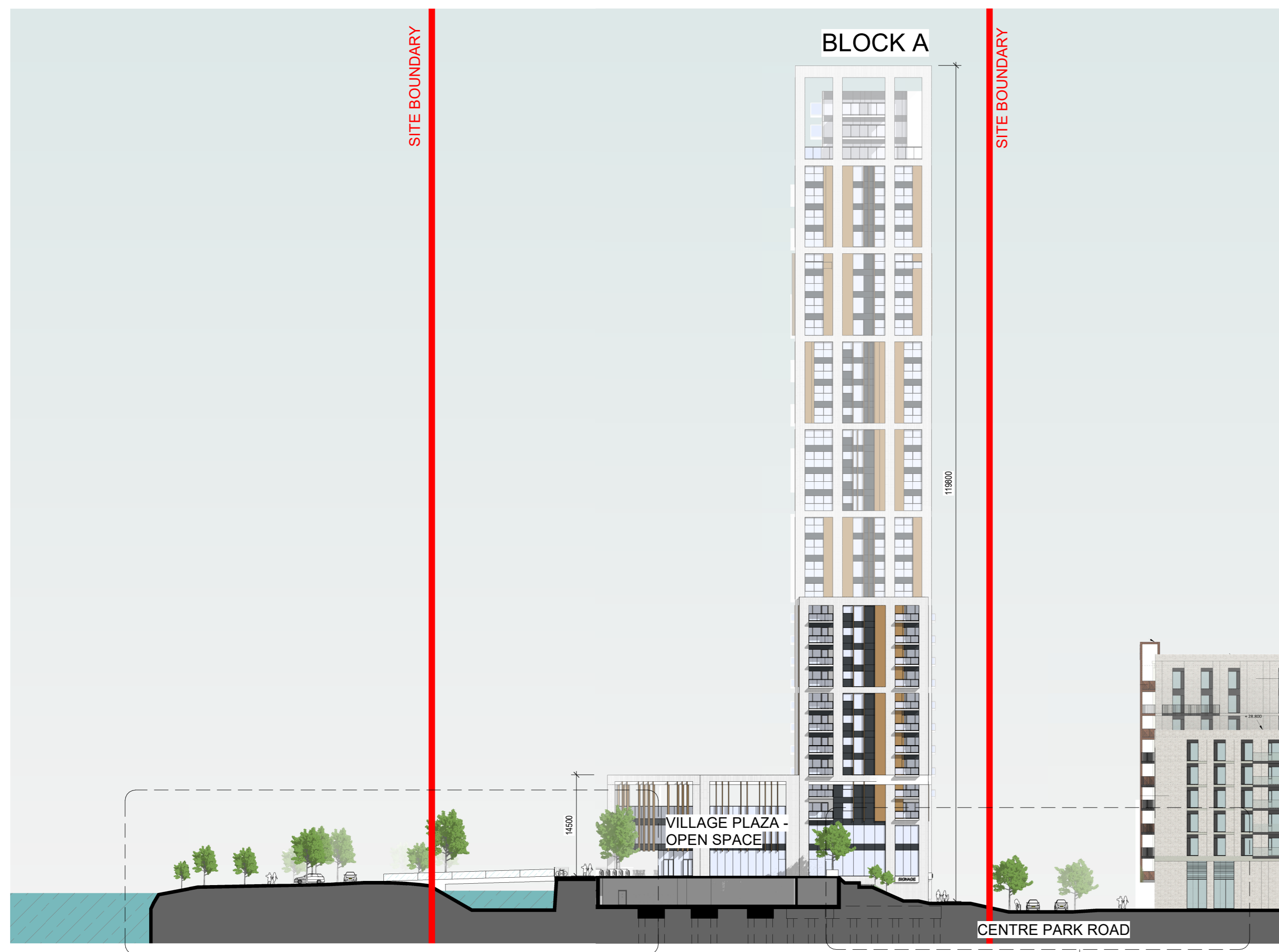
1 PROPOSED CONTEXTUAL SITE SECTION L-L 1:500
